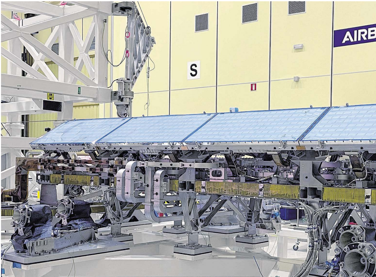
Wettersatellit MetOp-SG-B
